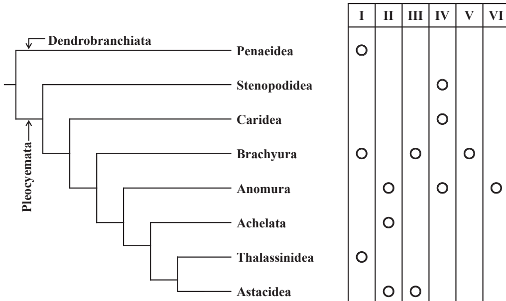
Fig. 2. Phylogenetic trees of decapods modified from Crandall et al. 4) (fig. 2) and hemocyte classification group (I-VI) of polyhemocytic decapods modified from Kondo et al. 1) (fig. 10).
