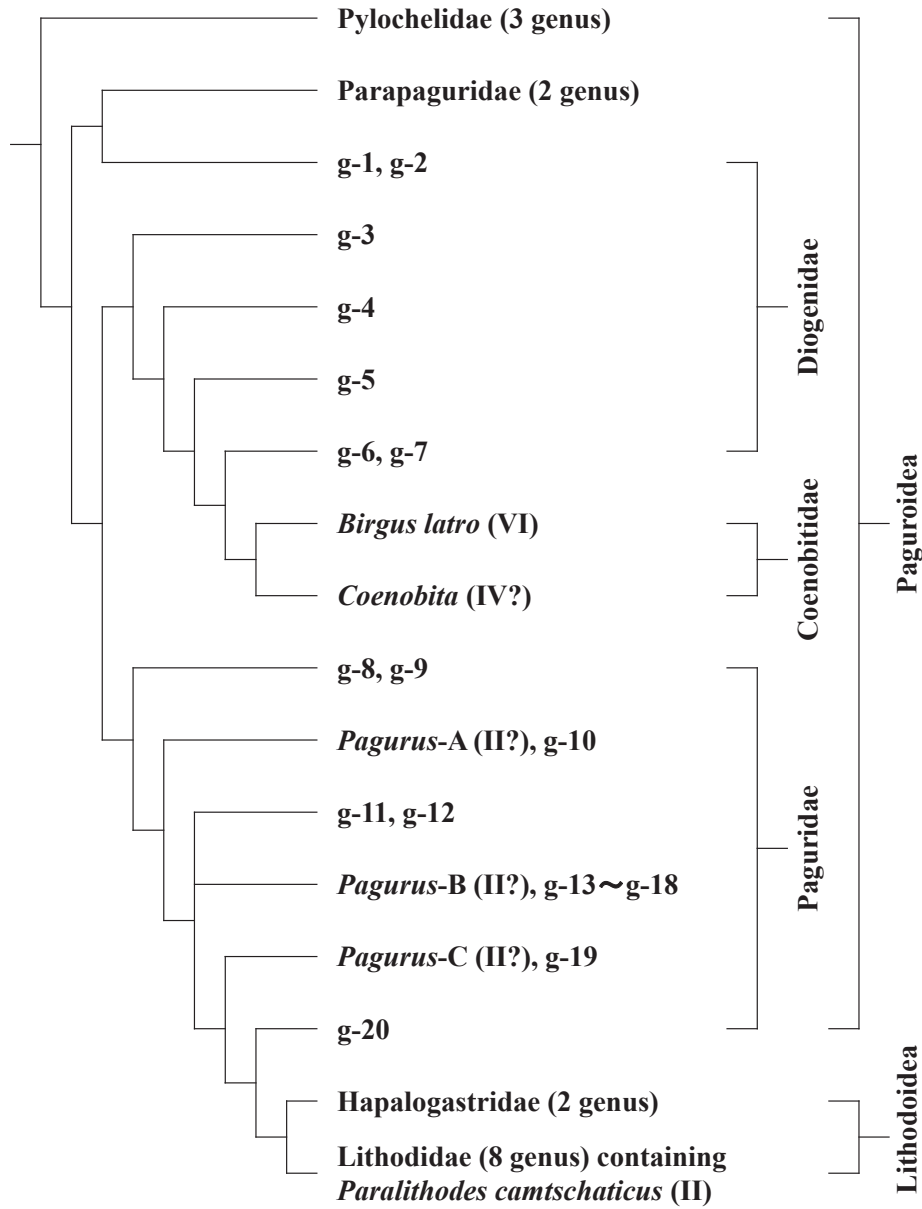
Fig. 3. Phylogenetic trees of anomuras (Paguroidea and Lithodoidea) modified and excerpted from Bracken-Grissom et al. 5) (fig. 1) and hemocyte classification group (II, IV, VI). g, genus; g-1~g-20, different genus each other; Pagurus-A ~ Pagurus-C , different species each other; II? & IV?, expected hemocyte classification group (because of the different species between Bracken-Grissom et al. 5) and our reports (present report and Kondo et al. 1) )).
