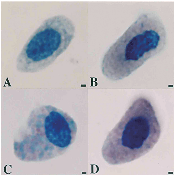
Fig. 1. Hemocytes of land hermit crab Coenobita cavipes (A & B; hemocyte classification group IV) and coconut crab Birgus latro (C & D; hemocyte classification group VI). A, chromophobic granulocyte (CG); B, eosinophilic granulocyte (EG); C, basophilic and eosinophilic granulocyte (BEG); D, eosinophilic granulocyte (EG). May-Grünwald stain. Bars=1 \mu\text{m} .
