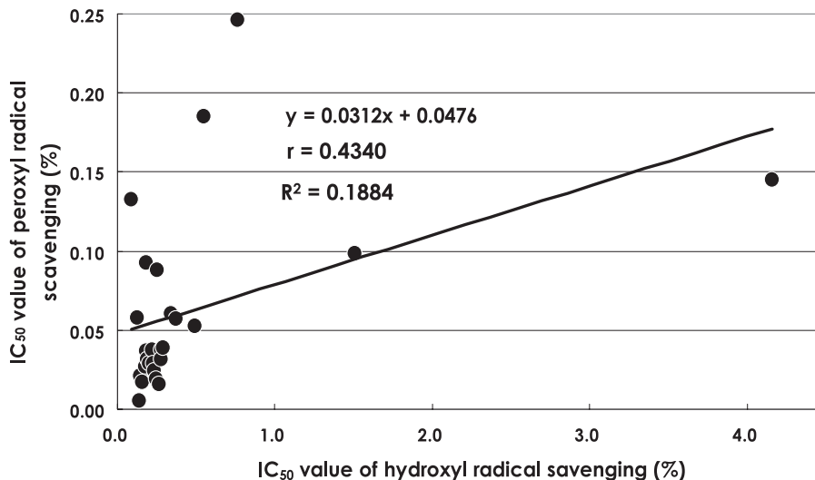
Fig. 4 . Relationship between IC_{50} value of peroxy radical scavenging and IC_{50} value of hydroxyl radical scavenging.
