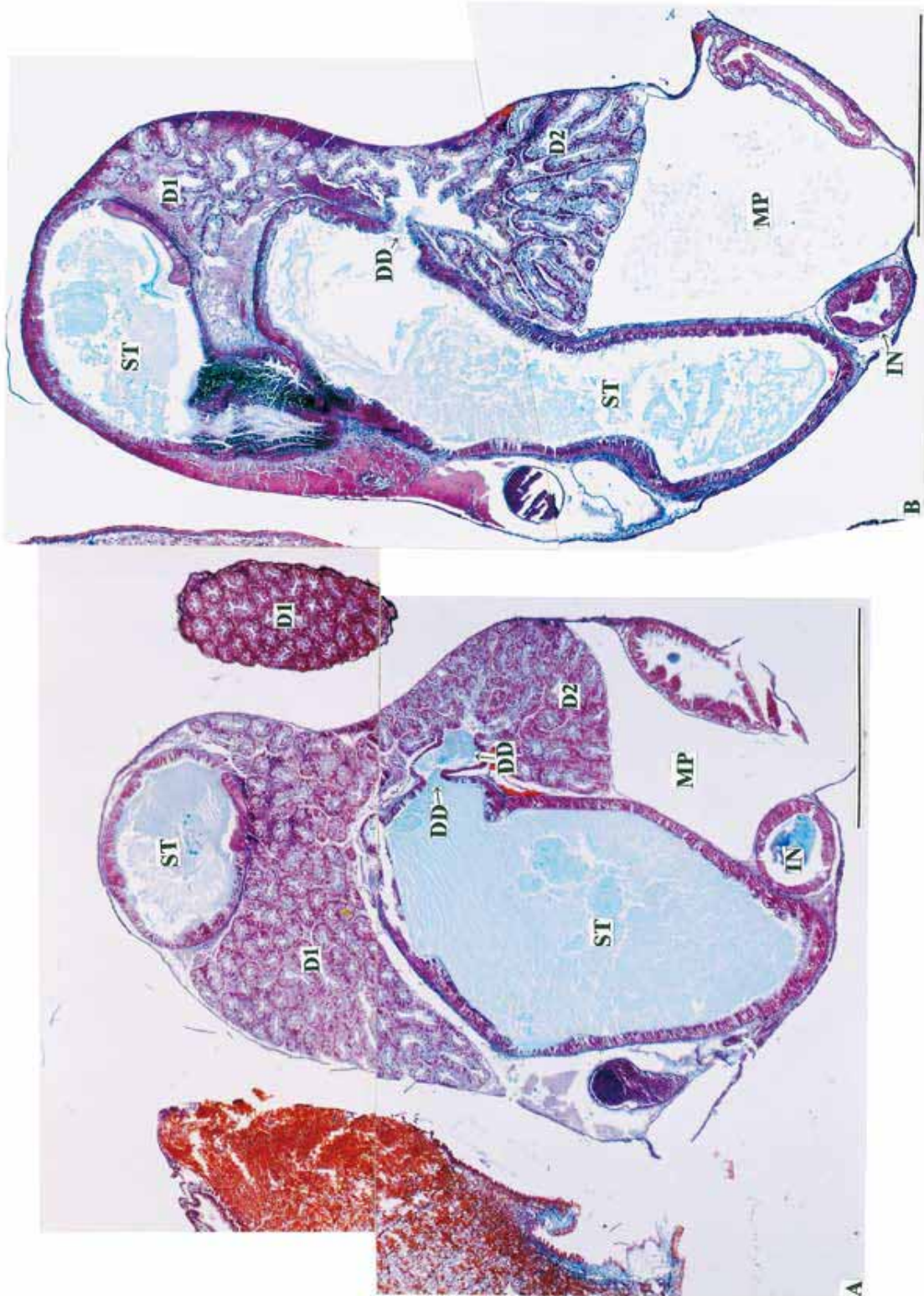
Fig. 4. Digestive diverticula of the mud snail. D 1 and D 2: digestive diverticula, DD: duet, MP: marsupium, ST: stomach, IN: intestine. Azan staining. Bars = 100 \mu m.
