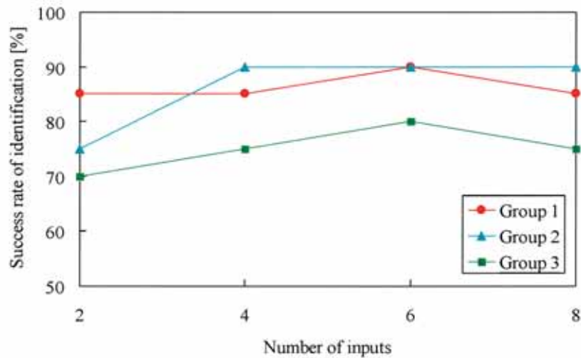
Fig. 7. Success rates of identification for shape data by aspect ratio.
