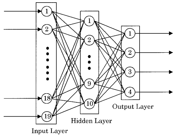
Fig. 2. Layered neural network for 19 shape data.
